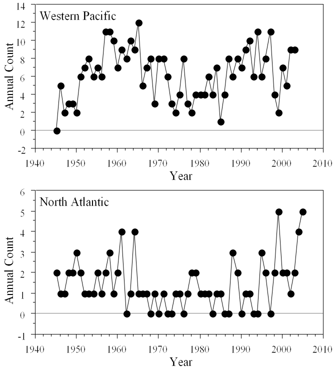
Figure 11 Category 4 and 5 Hurricanes
