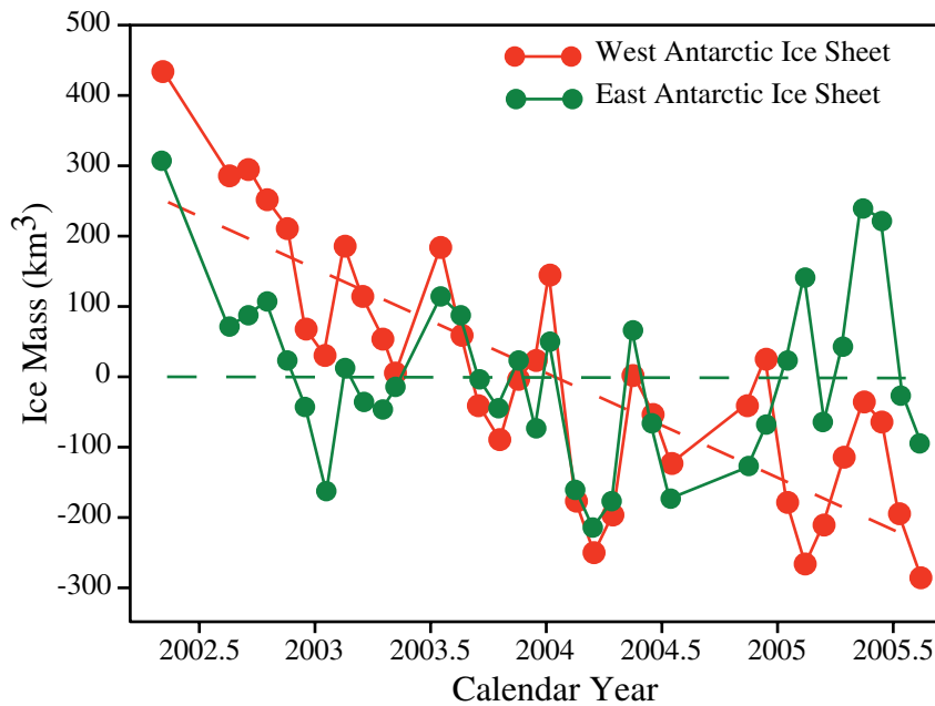
Ice mass variations over the West Antarctic Ice Sheet (red) and the East Antarctic Ice Sheet (green) as measured by a gravity-sensing satellite. Note that there are only 34 months of data. From Velicogna and Wahr, p. 1755.
