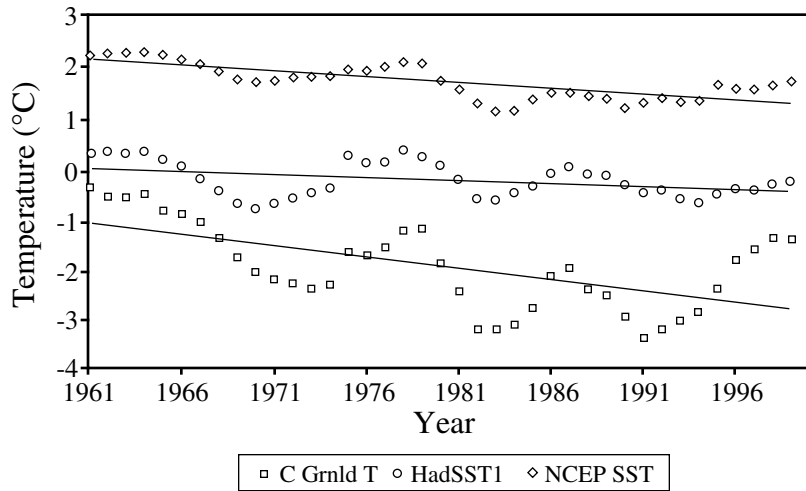
Figure 6 Composite Greenland Temperatures
