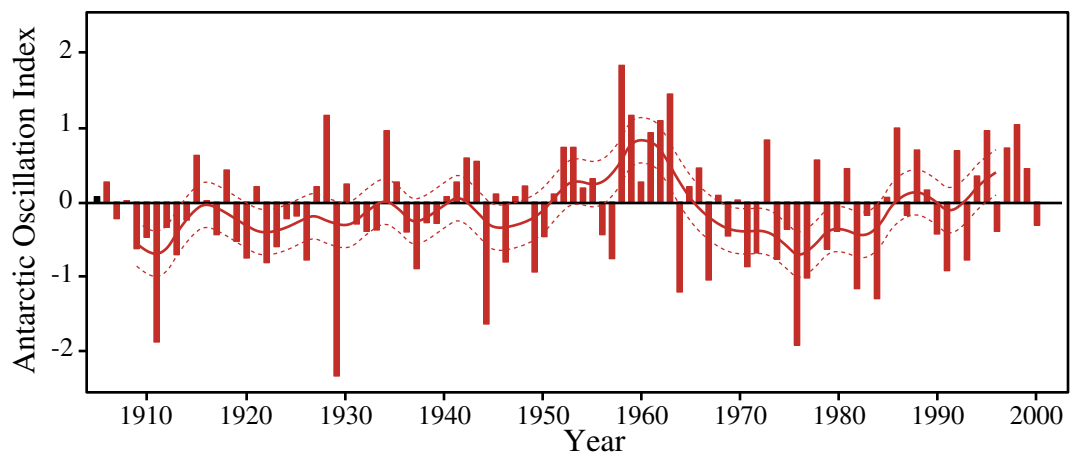
Figure 4 Reconstructed Variability of the SAM
