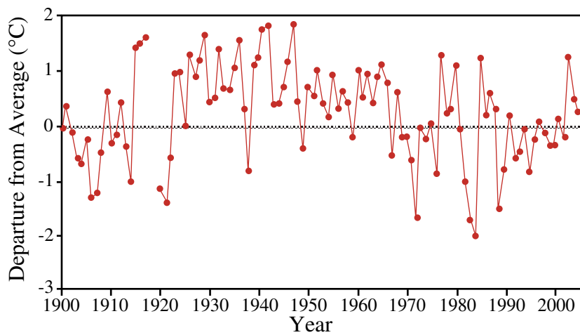
Figure 5 Temperature History from Southern Greenland, 1900–2005
