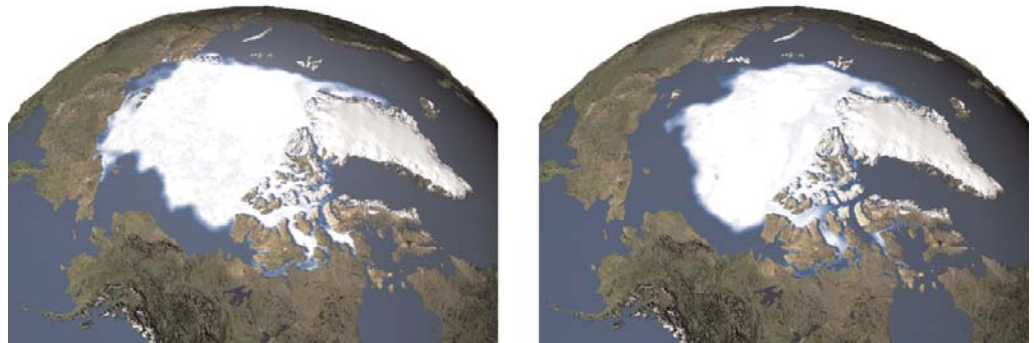
Figure 7 Extent of Arctic Sea Ice, 1979 and 2005
