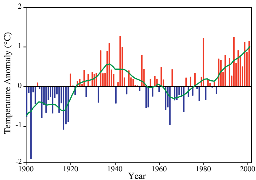
Figure 8b Surface Air Temperature Anomalies
