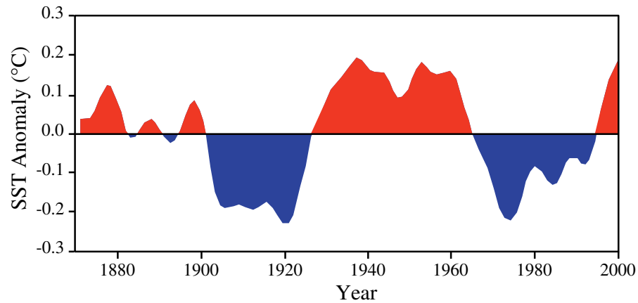
Figure 12 Time-History of AMO
