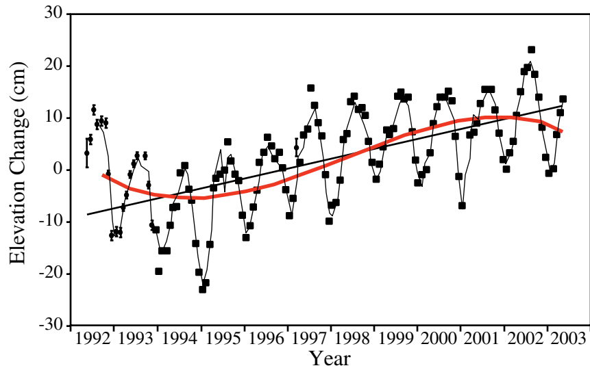
Figure 3 Ice Mass Change (elevation change) Observed over the East Antarctic Ice Sheet
