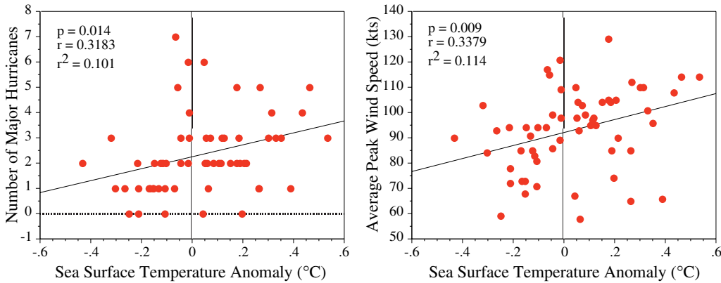
Observed relationship between sea-surface temperatures and two measures of hurricane intensity—the number of major hurricanes (Category 3, 4, and 5) each year (left), and the average peak wind speed in the five strongest storms in each year (right). From Michaels, Knappenberger, and Landsea, p. 5181.
