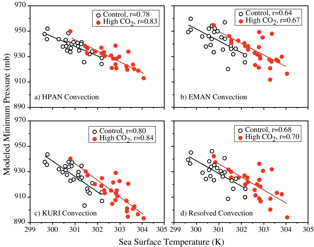
Relationship between sea-surface temperatures and hurricane intensity as measured by minimum central pressure (the lower the pressure, the stronger the storm) in the models used by Knutson and Tuleya.
