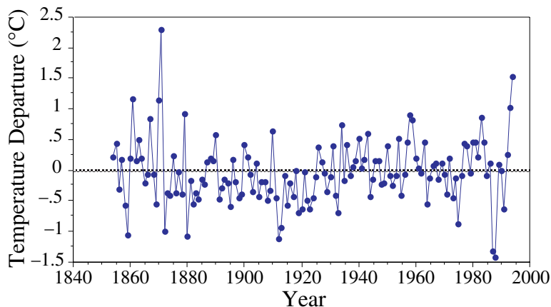
Figure 13 Temperature History of Northern Mexico
