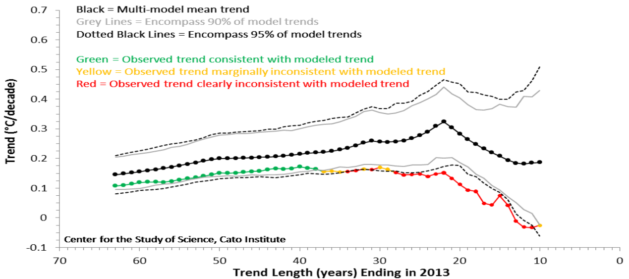
CAPTION: The annual average global surface temperature from 106 individual CMIP5 climate model runs forced with historical (+ RCP45 since 2006) forcings were obtained from the Climate Explorer website. Linear trends were computed through the global temperatures from each run, ending in 2013 and beginning each year from 1951 through 2004. The trends for each period (ranging in length from 10 to 62 years) were averaged across all model runs (black dots). The range containing 90 percent (grey lines), and 95 percent (dotted black lines) of trends from the 106 model runs is also indicated. The observed linear trends for the same periods were calculated from the annual average global surface temperature record compiled by the U.K. Hadley Center ( HadCRUT4 ) (colored dots). Observed trend values which were less than the 2.5 th percentile of the model trend distribution were colored red, observed trend values which were between the 2.5 th and the 5 th percentile of the model trend distribution were colored yellow, and observed trend values greater than the 5 th percentile of the model trend distribution were colored green.
